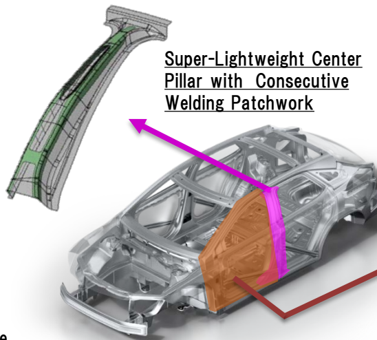
Aluminum/Steel Multi-Material Door (Lightweight & Saving Cost)
