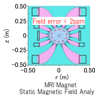
Control Technology for High Voltage and High Magnetic Field
