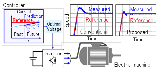
Control Technology for Driving Electric Motors (Predictive Control)
