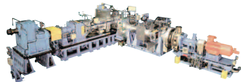
図1 混練造粒装置LCM450H Fig. 1 LCM mixer-pelletizer system for resin : LCM450H
