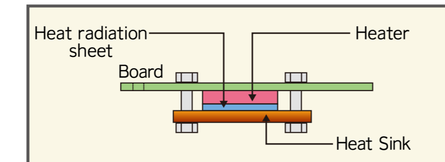
4 The heat sink and lid made of Kobe Honetsu are mounted
