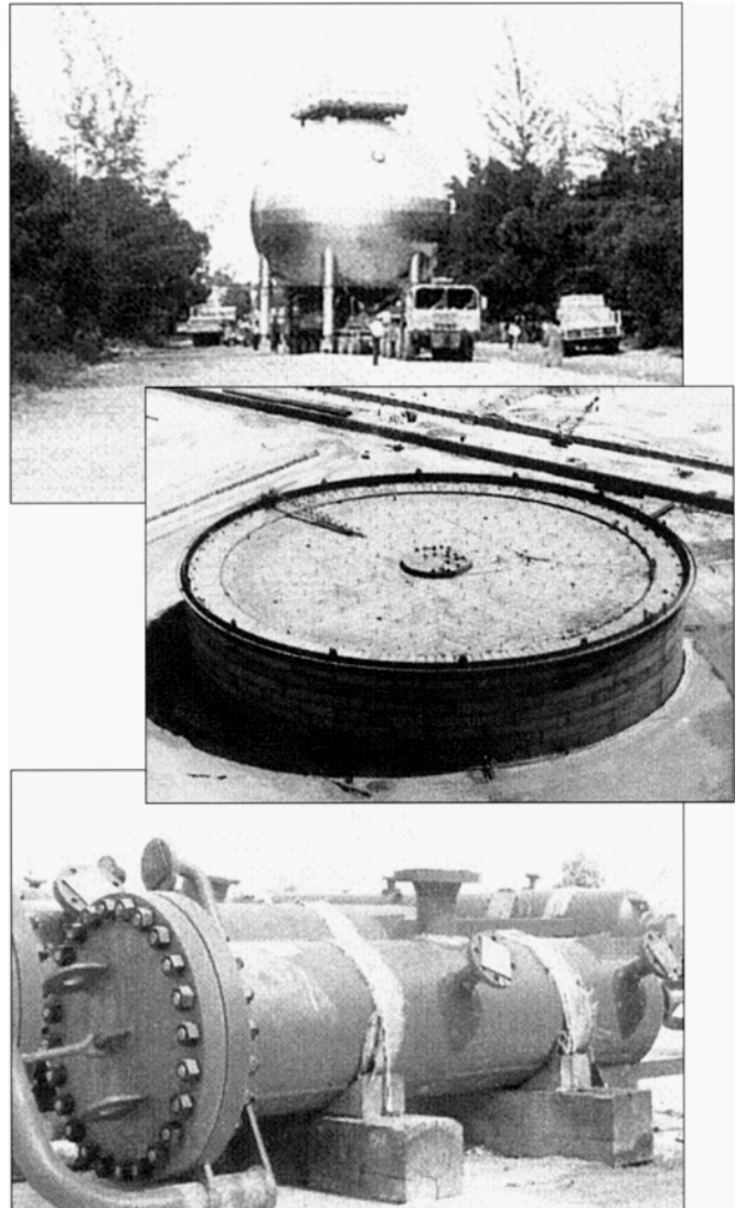
A 360-m 3 shop-erected propane sphere ready for shipment to Singapore (Top); An 800,000 bbl floating roof tank constructed in Kalimantan (Middle); A variety of pressure vessels ready for loading (Bottom)
