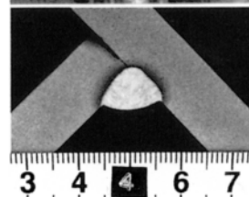
Figure 3. Macrostructure of the central cross section of the weld shown in Figure 2, having sufficient penetration and smooth fusion with the base metal with no undercut
