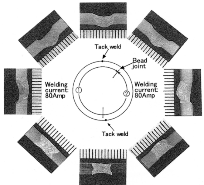
Figure 2. Macrostructure of TGX-308L welds made on a 304-type stainless steel tube (4T X 50 mmØ) in horizontally fixed position (5G position per ASME). The terminal of the 2nd pass was joined with the terminal of the 1st pass at the point between the 1 o'clock position and the 2 o'clock position.
