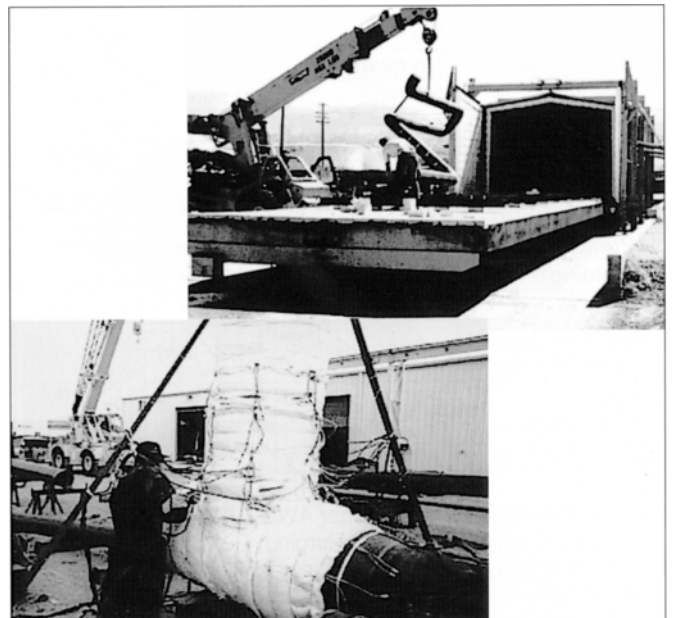
Figure 2. (Top): A computer-controlled furnace (Photo source: Pipe Fabrication & Supply, USA) (Bottom): Local annealing of a tee (Photo source: Technical Heat Treatment Services, Canada)
