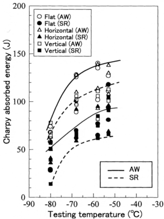
Figure 3. Charpy impact test results of DW-55LSR weld metals in the following conditions:
