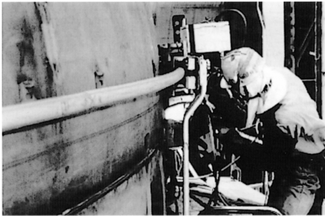
Figure 1. An example of the applications for DW-55LSR: an LPG tank of an LPG carrier with a maximum plate thickness of 40 mm requiring local stress relief annealing
