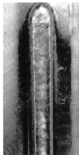
Figure 2. Bead appearance made in straight-run vertical-up fillet welding, having a smooth regular surface with no undercut ▪ Brand: DW-81B2 ▪ Wire size: 1.2 mmØ ▪ Welding condition: 220A (DCEP)-25V ▪ Shielding gas: 75%Ar + 25%CO 2 25 liter/min ▪ Leg length: Approx. 7 mm
