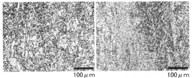
Figure 1. Typical microstructure of weld metals (Shielding gas: 75%Ar+25%CO 2 , PWHT: 690 C x 1hr)
