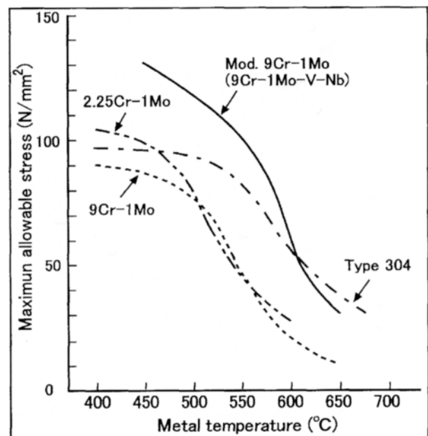
Figure 1. A comparison between 9Cr-1Mo-V-Nb and other steels on the maximum allowable stress for high-temperature equipment over a range of metal temperatures
