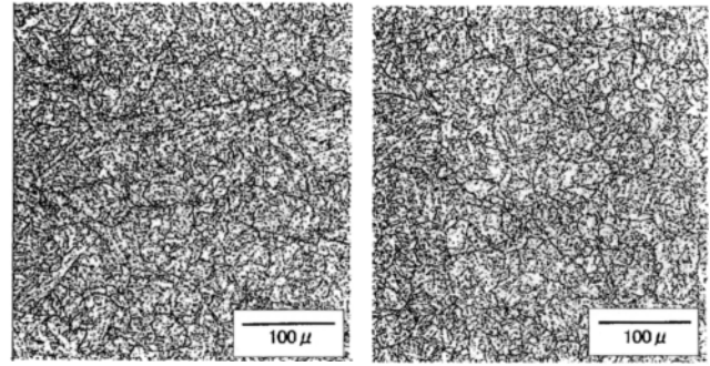
Photo 3. CM-9Cb deposits homogeneous microstructure consisting of tempered martensite with the absence of polygonal ferrite after PWHT (750°C x 5h), exhibiting a dendritic zone in the left and a pass-to-pass tempered zone in the right
