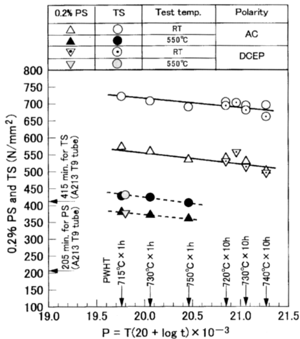
Figure 2. Mechanical properties of CM-9 (5.0Ø) deposited metal in flat position as a function of Rarson & Miller temper parameter (P) in PWHT
