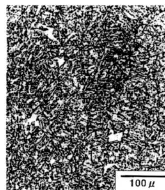
Photo 2. A microstructure of CM-9 deposited metal exhibits fine, tempered martensite without the precipitation of coarse ferrite (PWHT: 750°C x 1h)
