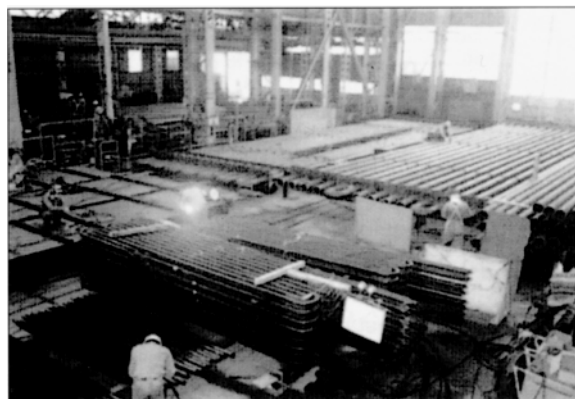
Photo 4. 9Cr steels are indispensable for superheater tubes, reheater tubes and steam headers of coal-fired steam boilers in the trend of higher steam conditions (Photo courtesy: Nagasaki Kogyosho Co., Ltd., Japan)
