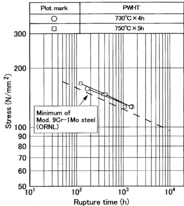
Figure 5. Creep rupture strength of CM-9Cb (4.0Ø) deposited metal in flat position, satisfying the minimum rupture strength of Mod. 9Cr-1Mo steel
