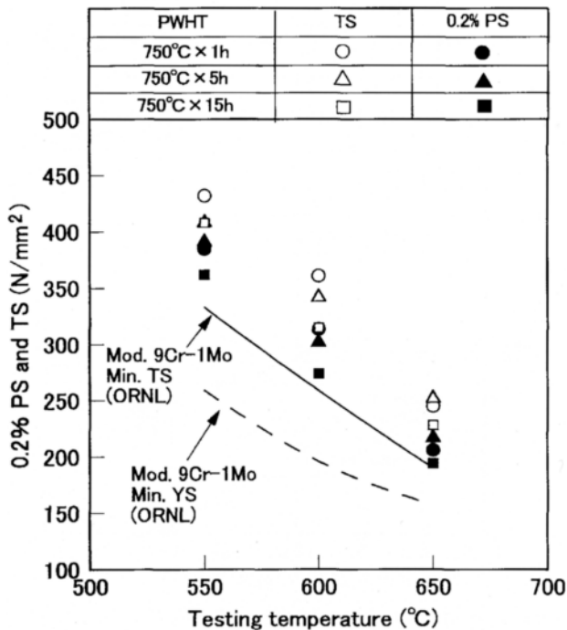
Figure 4. High-temperature strength of CM-9Cb (4.0Ø) deposited metal in flat position, satisfying the minimum strength of Mod. 9Cr-1Mo steel within the given PWHT conditions
