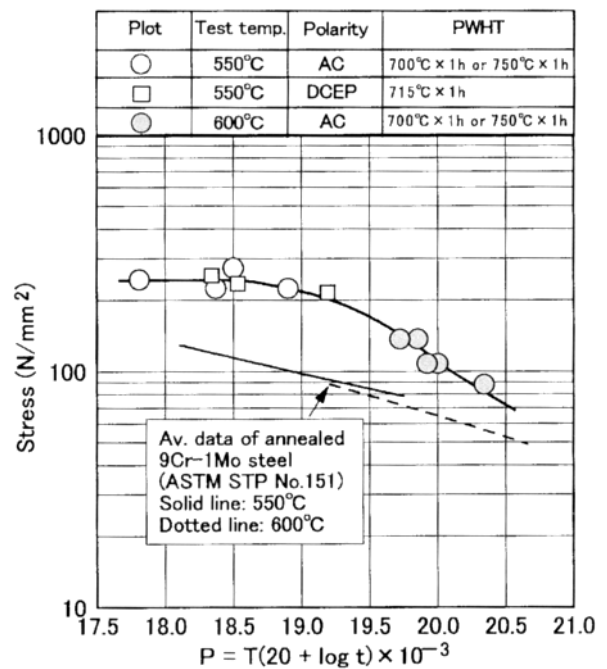
Figure 3. A master creep curve of CM-9 (5.0 Ø) deposited metal in the flat position as a function of Rarson & Miller parameter in creep rupture testing
