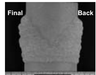
Figure 2: Macrostructure in 2G position
