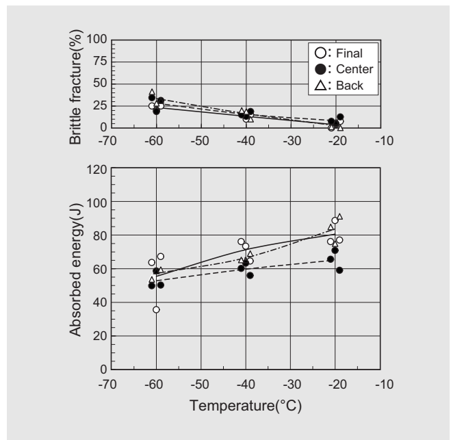
Figure 4: Notch toughness transition curve in 2G position
