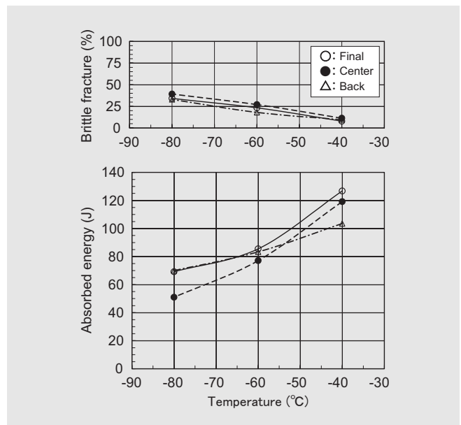
Figure 3: Notch toughness transition curve in 1G position
