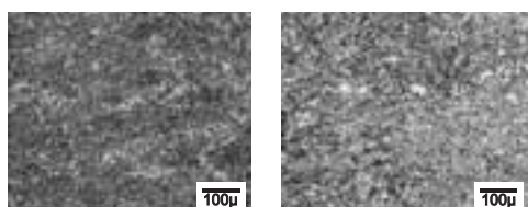
Figure 1: Ti-B micro-alloyed fine microstructures of DW-62L (left) and DW-A62L (right) weld metals.
