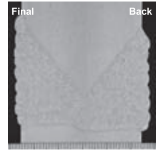
Figure 2: Macrostructure in 2G position
