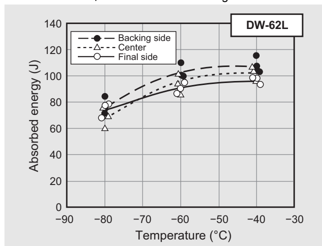
Figure 2: Charpy impact absorbed energies of weld metals tested with 60mm thick double-V groove joints and 1.2 mmφ wires in vertical welding.
