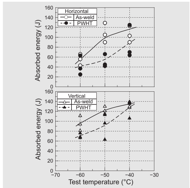
Figure 2: Absorbed energies in Charpy impact testing of DW-A81Ni1 weld metal in the as-welded and PWHT (580°C x 2h) conditions (Base metal: 50mm thick FH36; Groove: double bevel; Specimen location: final side).
