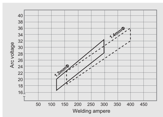
Figure 4: Proper range of welding amperage and arc voltage with DW-55L (1.2 and 1.4 mm \phi ).
