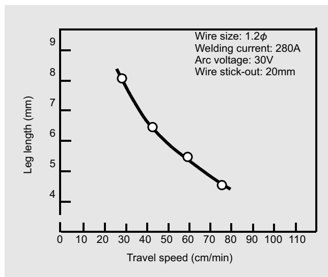
Figure 2: Fillet leg length vs. travel speed in uses of DW-55E and DW-A55E in single pass horizontal fillet welding.
