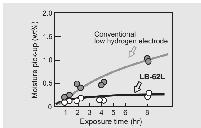
Figure 5: Test results of LB-62L and conventional low-hydrogen electrode on moisture pick-up under the controlled atmosphere: 30°C x 80%R.H.
