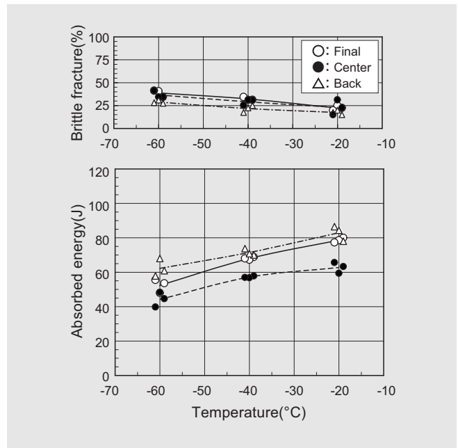
Figure 3: Notch toughness transition curve in 3G position
