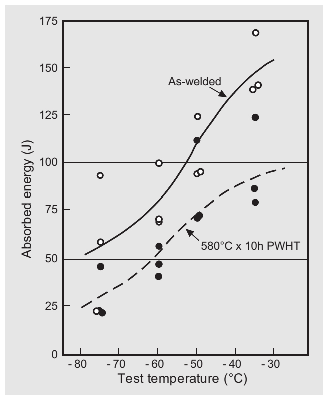
Figure 4: Effect of postweld heat treatment on impact absorbed energy of LB-62L (4.0 mmφ) weld metal (Power source: DCEP; Heat input: av. 3.9 kJ/mm; Welding position: Vertical up; Base metal: A537 Cl.2; Groove preparation: double V).
