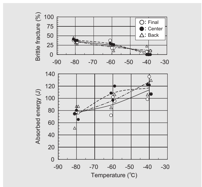
Figure 4: Notch toughness transition curve in 2G position
