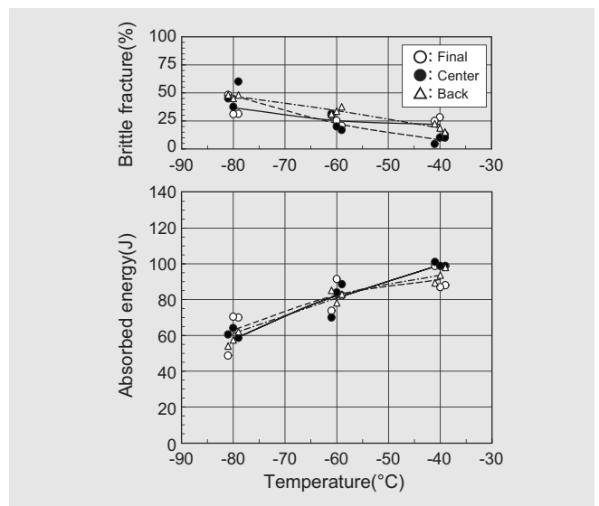
Figure 3: Notch toughness transition curve in 3G position
