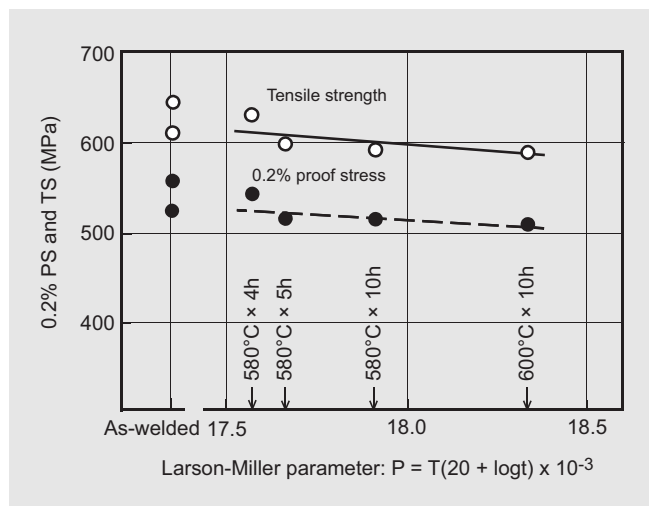
Figure 3: Strength of LB-62L (5.0 mmφ) all-deposited metal vs. PWHT parameter (Power source: DC-EP, Heat input: av. 1.9 kJ/mm, Welding position: flat).
