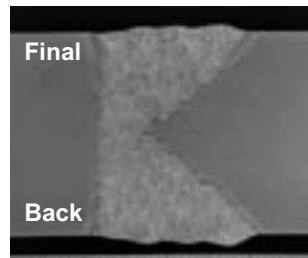
Figure 1: Macrostructure in 1G position
