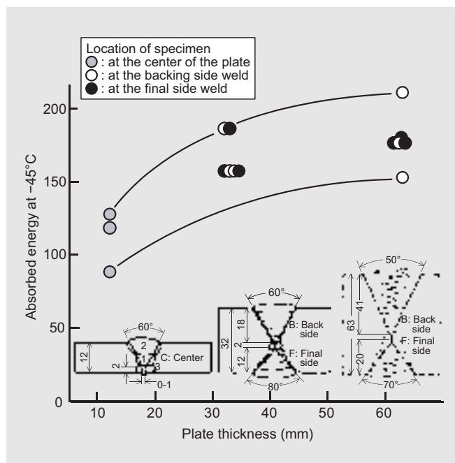
Figure 2: Charpy impact test results of LB-52NS (4 mm \phi ) weld metals in vertical-up AC welding (interpass temperature: 100–150°C).
